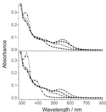
Figure 3. UV/Vis absorption spectra of 30 \mu\text{M} of 1 (top) and 2 (bottom) in the absence of polymers ( \blacksquare ) and in the presence of the 180 \mu\text{M} of polyacrylate ( \bullet ), poly(vinyl sulfonate) ( \blacktriangle ), and poly(4-styrene sulfonate) ( \star ) in buffer (5 mM Tris, 10 mM NaCl, pH 7.5) solution.
