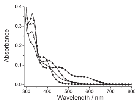
Figure 2. UV/Vis absorption spectra of 2 in the absence (●) and in the presence (★) of 1 M NaCl, and 3 in the absence (▲) and in the presence (■) of 1 M NaCl in buffer (5 mM Tris, 10 mM NaCl, pH 7.5) solution.
