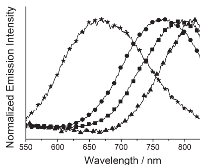
Figure 4. Normalized emission spectra of 30 \mu\text{M} of 1 ( \blacksquare ), 2 ( \bullet ), 3 ( \blacktriangle ) and 4 ( \star ) mixed with 180 \mu\text{M} of polyacrylate in buffer (5 mM Tris, 10 mM NaCl, pH 7.5) solution.
