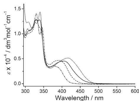
Figure 1. UV/Vis spectra of 30 \mu\text{M} of complexes 1 (—), 2 (---), 3 (.....) and 4 (-.-.-) in buffer- \text{CH}_3\text{CN} solvent mixture (Medium: 5 mM Tris-HCl, 10 mM NaCl, pH 7.5, 40% \text{CH}_3\text{CN} ).
