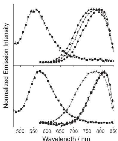
Figure 5. Normalized emission spectra of 30 \mu\text{M} of 1 (top) and 3 (bottom) in the absence of polymers (■) in buffer– \text{CH}_3\text{CN} solvent mixture and in the presence of the 180 \mu\text{M} of polyacrylate (●), poly(vinyl sulfonate) (▲), and poly(4-styrene sulfonate) (☆) in buffer (5 mM Tris, 10 mM NaCl, pH 7.5) solution.
