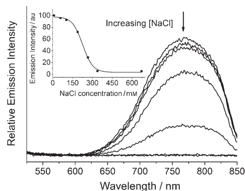
Figure 6. Emission spectra of 30 \mu\text{M} of complex 2 + 180 \mu\text{M} of polyacrylate, 5 mM Tris-HCl, 10 mM NaCl, pH 7.5, with increasing concentration of NaCl added. Inset: plot of emission intensity at 771 nm as a function of NaCl concentration.
